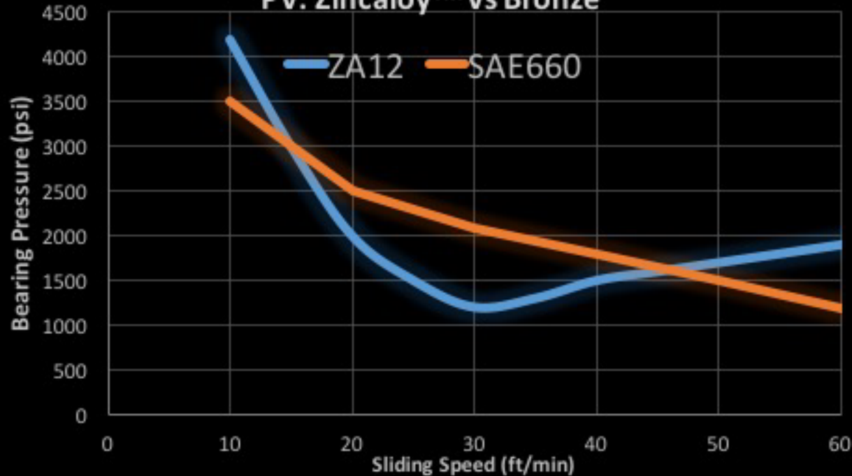
PV: ZincaIoy™ vs Bronze
